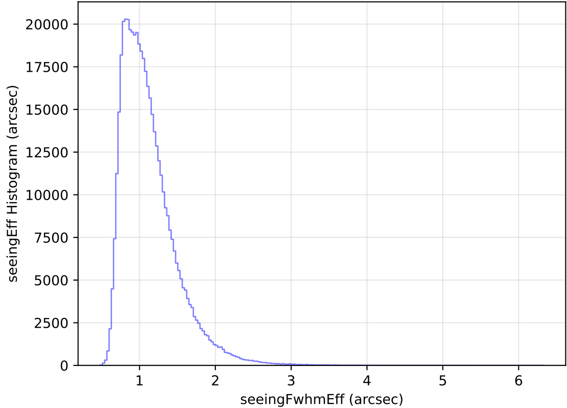
too_elab_heavy_r64_d3_ugrizy_v3.4_10yrs All sky r band: seeingEff Histogram
