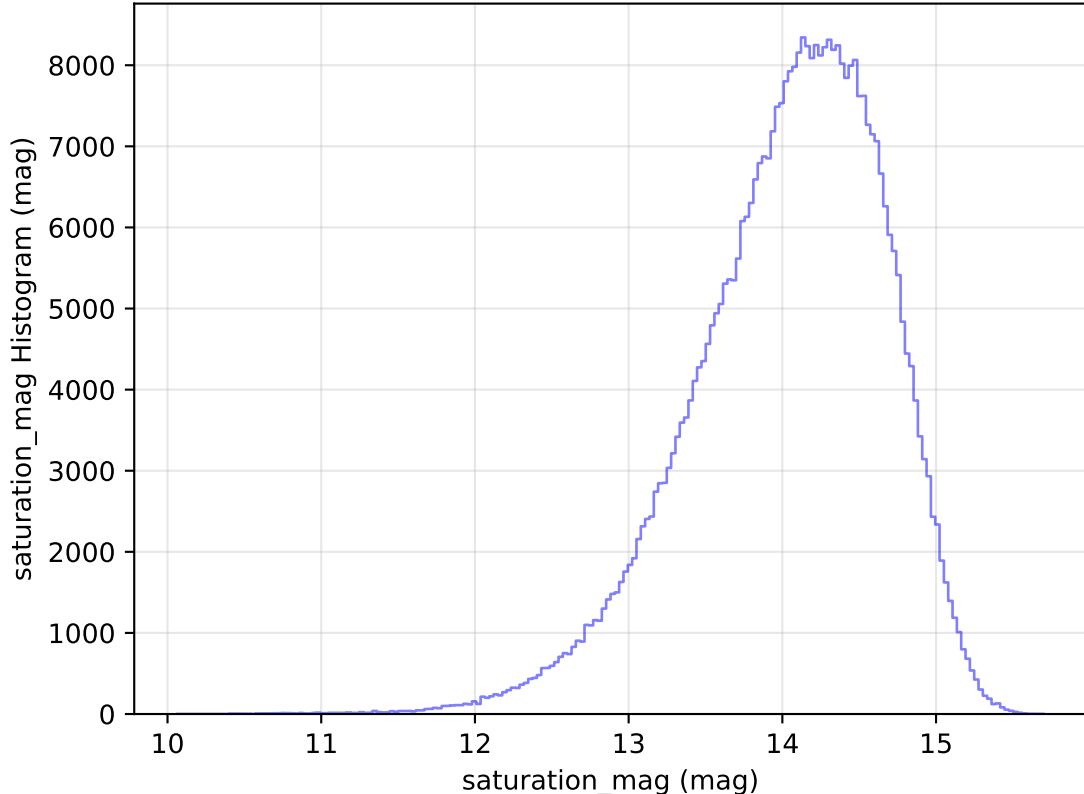
too_elab_heavy_r64_d3_ugrizy_v3.4_10yrs WFD z band: saturation_mag Histogram
