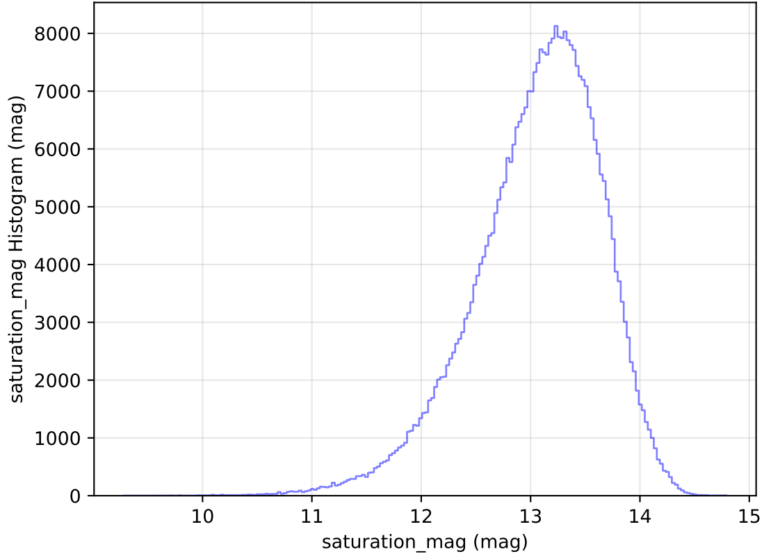
too_elab_heavy_r64_d3_ugrizy_v3.4_10yrs WFD y band: saturation_mag Histogram
