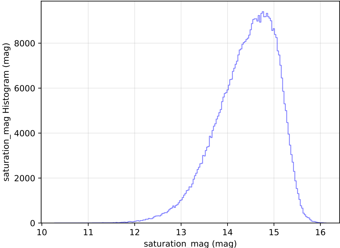
too_elab_heavy_r64_d3_ugrizy_v3.4_10yrs WFD i band: saturation_mag Histogram
