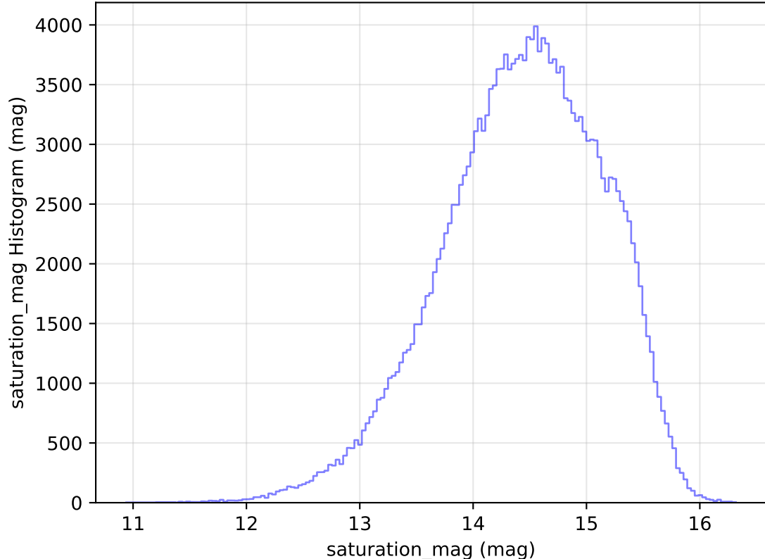
too_elab_heavy_r64_d3_ugrizy_v3.4_10yrs WFD g band: saturation_mag Histogram
