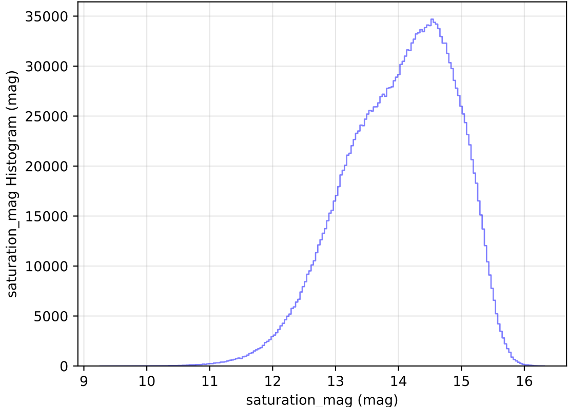
too_elab_heavy_r64_d3_ugrizy_v3.4_10yrs WFD all bands: saturation_mag Histogram
