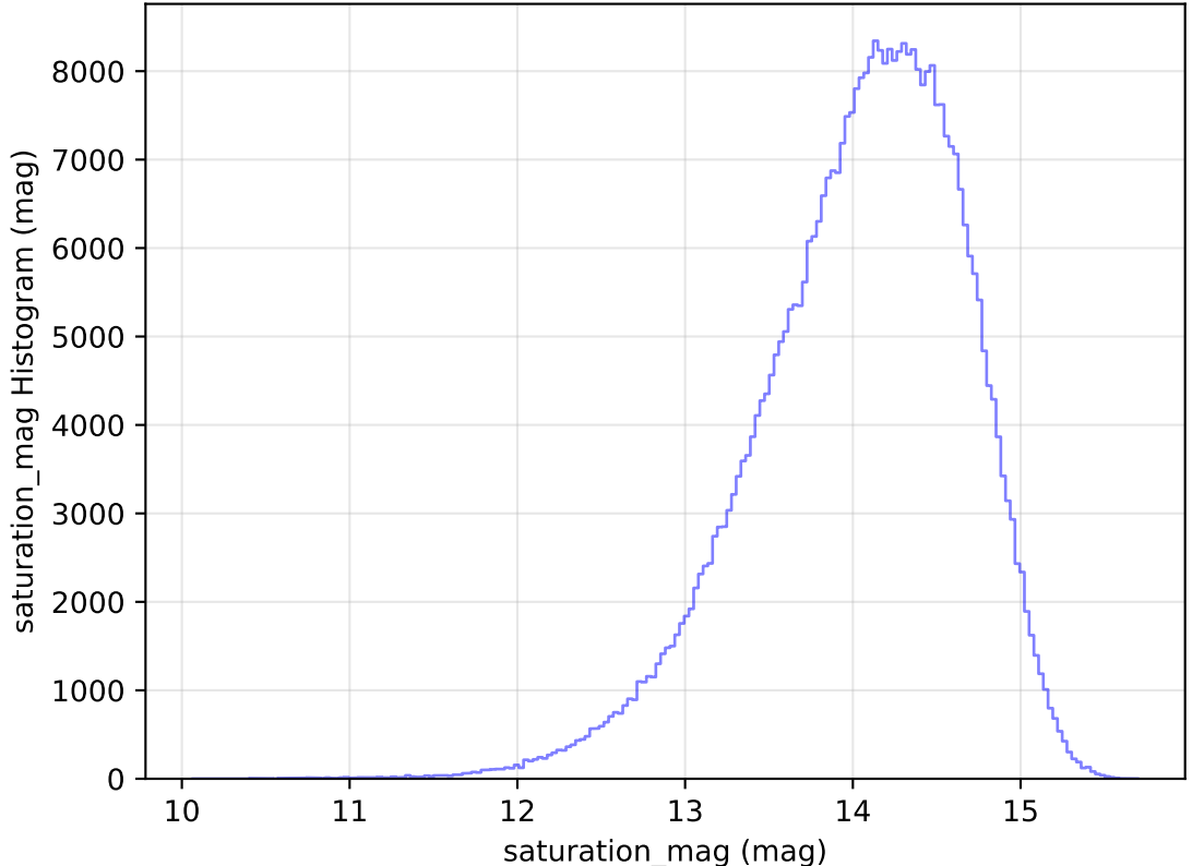
too_elab_heavy_r64_d3_ugrizy_v3.4_10yrs All sky z band: saturation_mag Histogram
