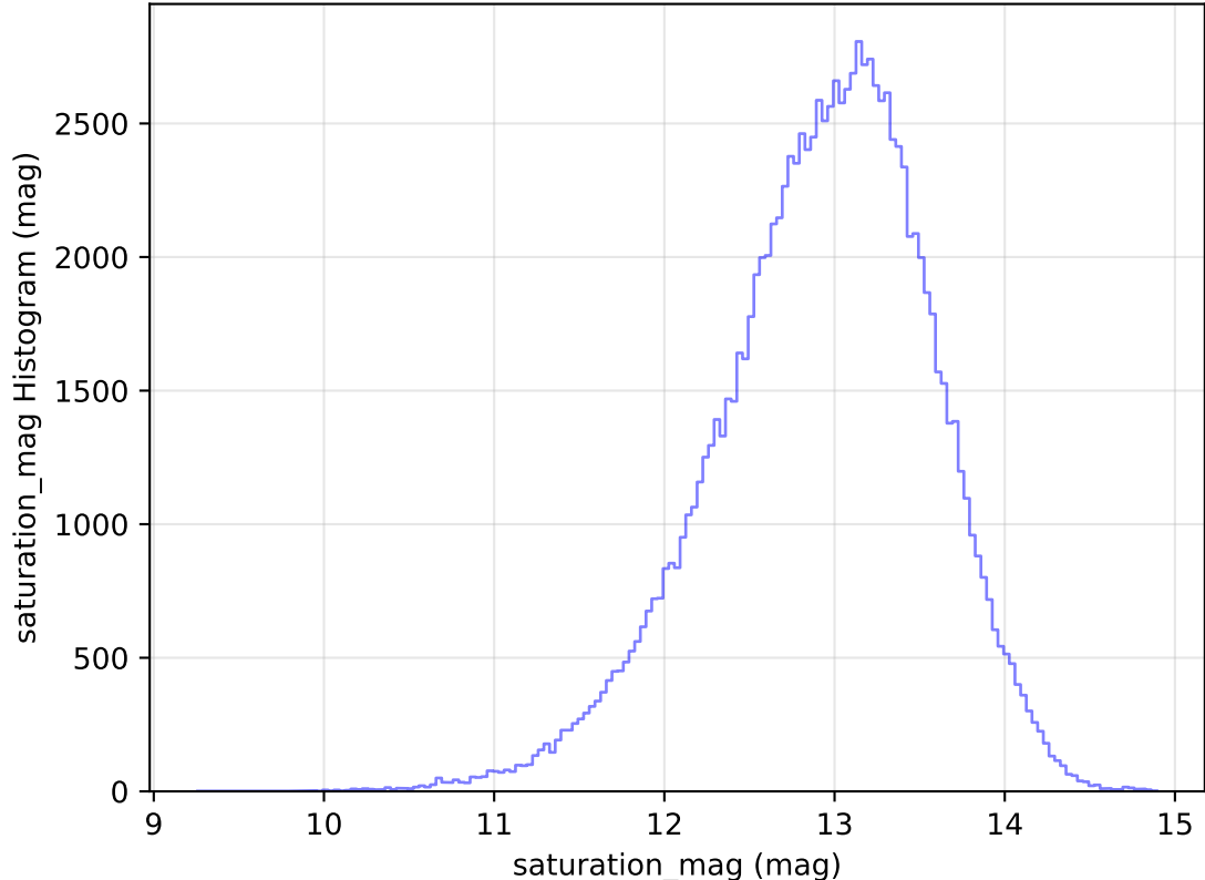
too_elab_heavy_r64_d3_ugrizy_v3.4_10yrs All sky u band: saturation_mag Histogram
