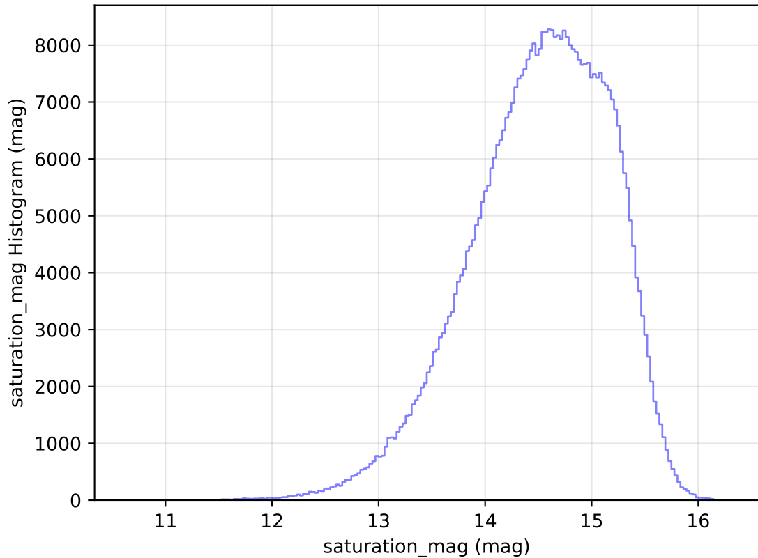
too_elab_heavy_r64_d3_ugrizy_v3.4_10yrs All sky r band: saturation_mag Histogram
