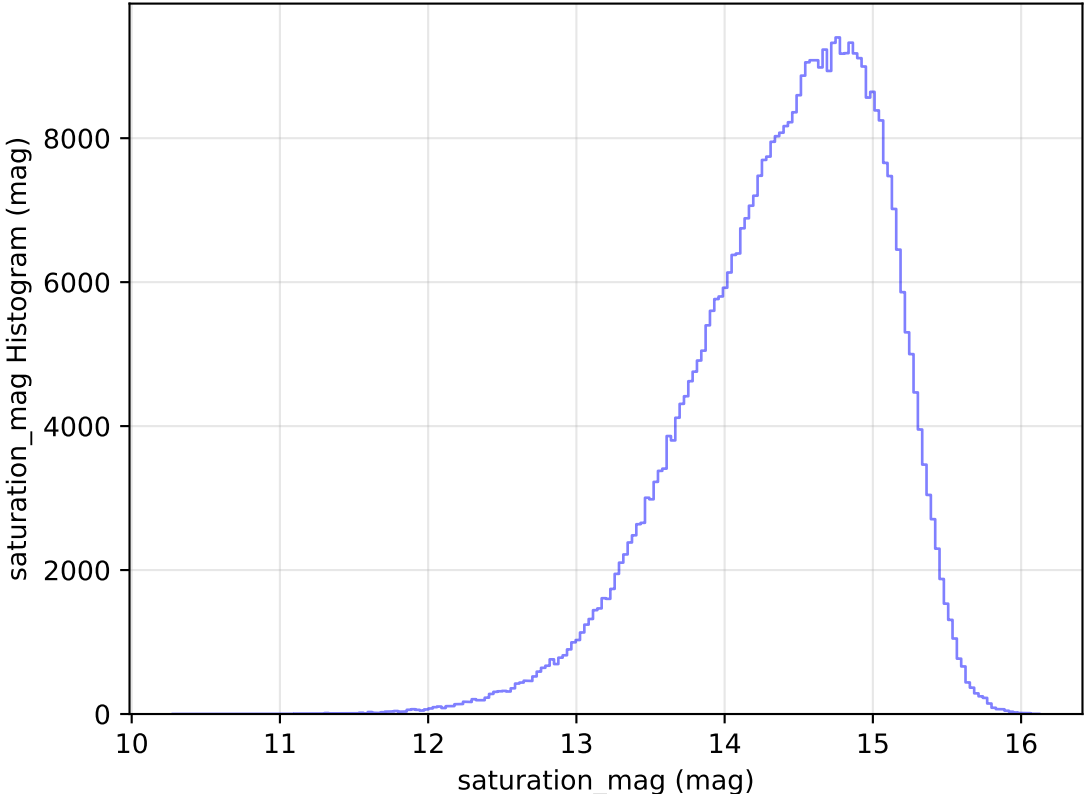
too_elab_heavy_r64_d3_ugrizy_v3.4_10yrs All sky i band: saturation_mag Histogram
