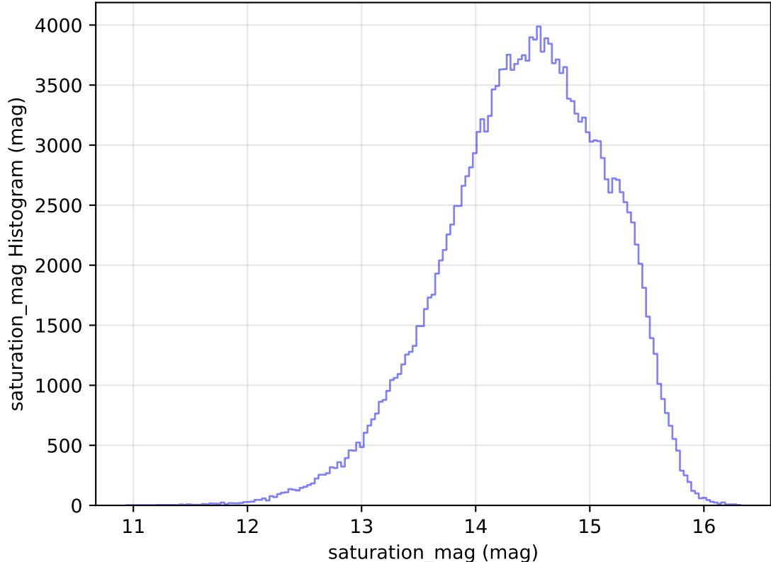
too_elab_heavy_r64_d3_ugrizy_v3.4_10yrs All sky g band: saturation_mag Histogram
