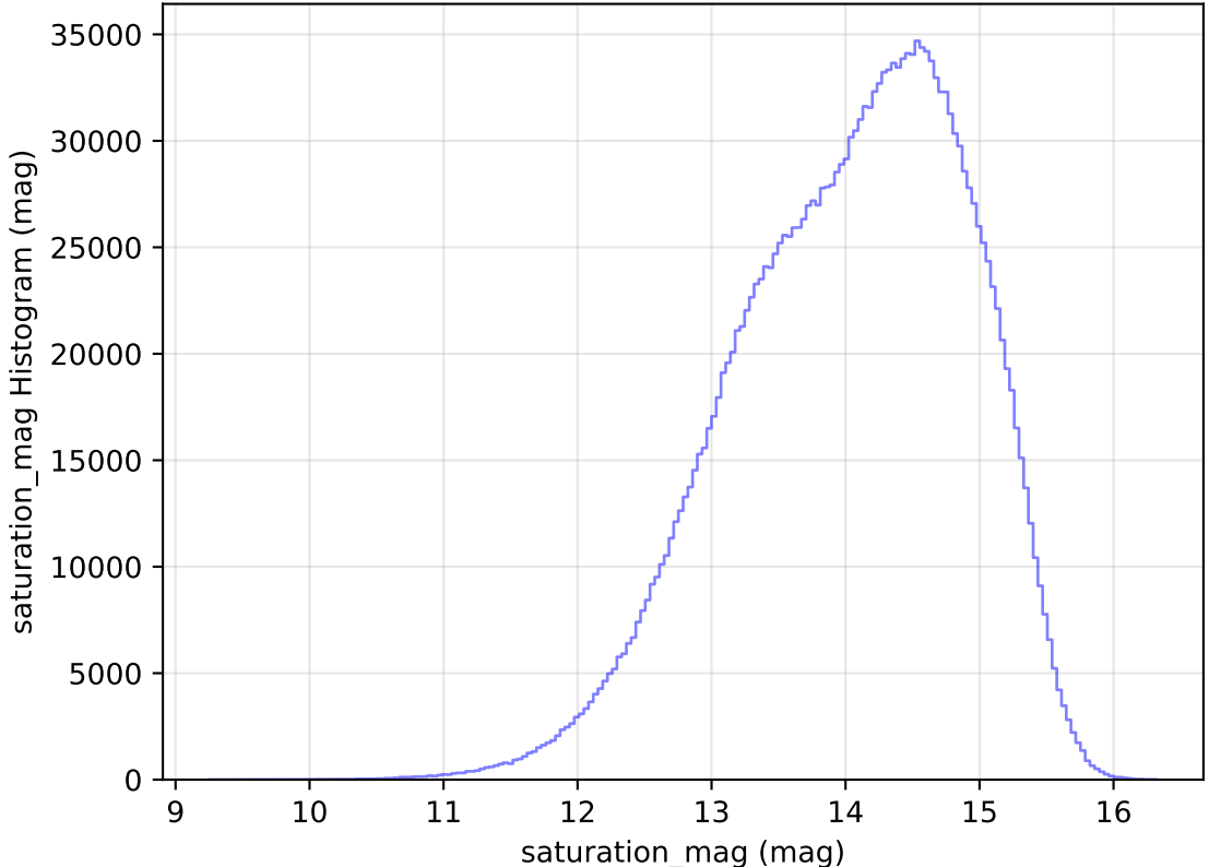
too_elab_heavy_r64_d3_ugrizy_v3.4_10yrs All sky all bands: saturation_mag Histogram
