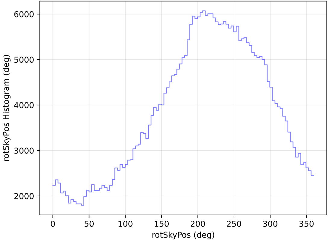
too_elab_heavy_r64_d3_ugrizy_v3.4_10yrs WFD y band: rotSkyPos Histogram
