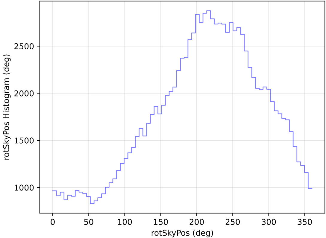
too_elab_heavy_r64_d3_ugrizy_v3.4_10yrs WFD u band: rotSkyPos Histogram
