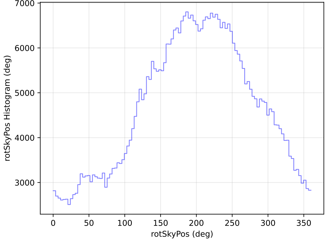
too_elab_heavy_r64_d3_ugrizy_v3.4_10yrs WFD r band: rotSkyPos Histogram
