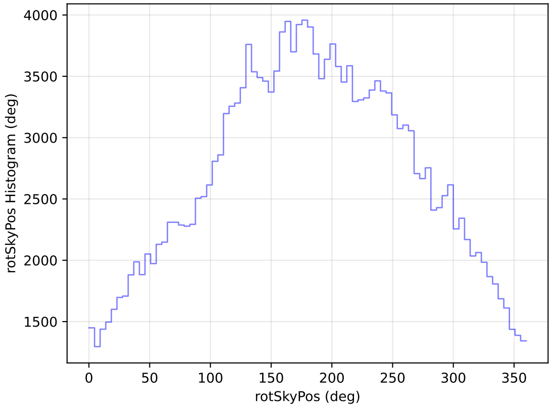
too_elab_heavy_r64_d3_ugrizy_v3.4_10yrs WFD g band: rotSkyPos Histogram
