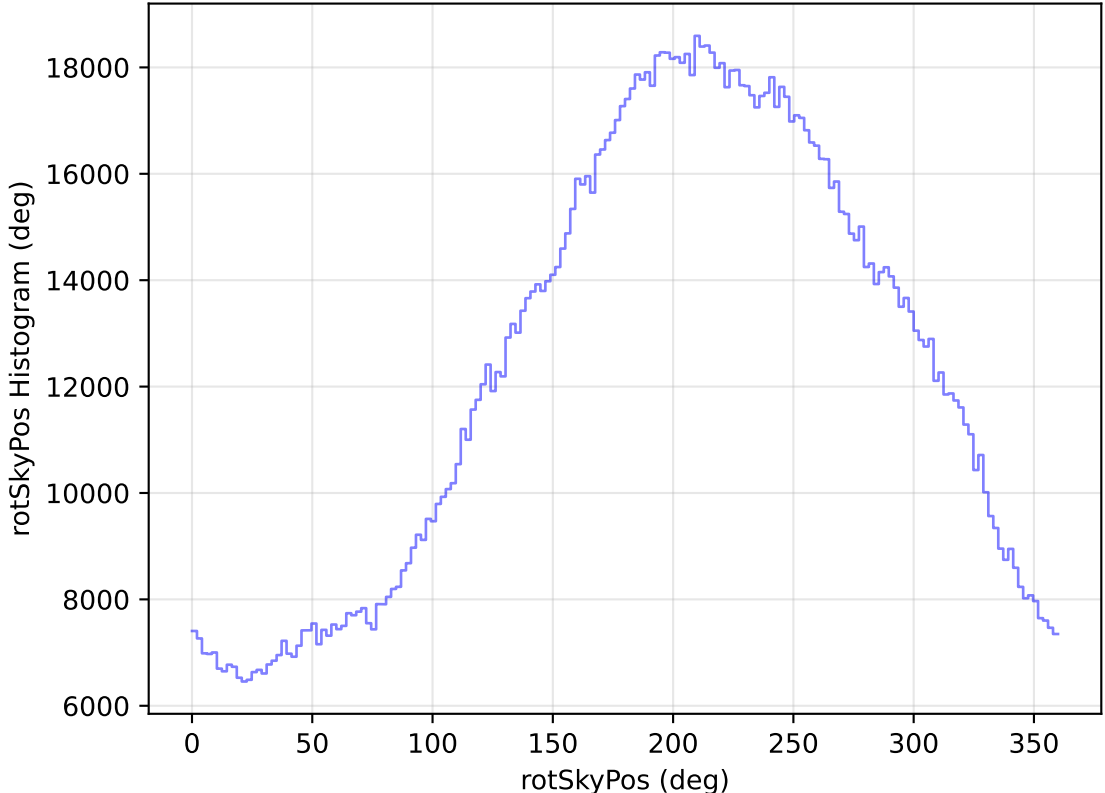
too_elab_heavy_r64_d3_ugrizy_v3.4_10yrs WFD all bands: rotSkyPos Histogram
