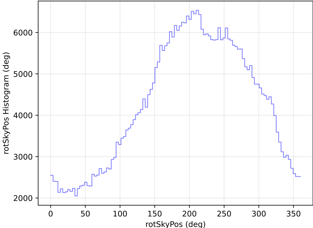
too_elab_heavy_r64_d3_ugrizy_v3.4_10yrs All sky z band: rotSkyPos Histogram
