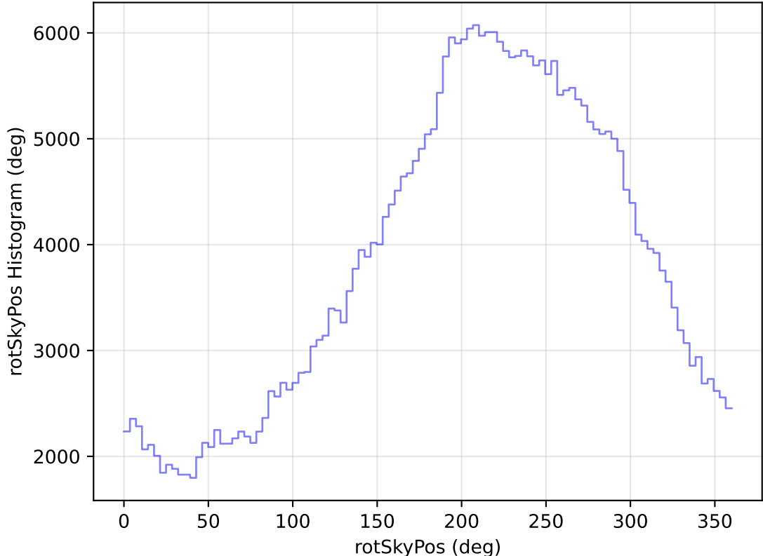
too_elab_heavy_r64_d3_ugrizy_v3.4_10yrs All sky y band: rotSkyPos Histogram
