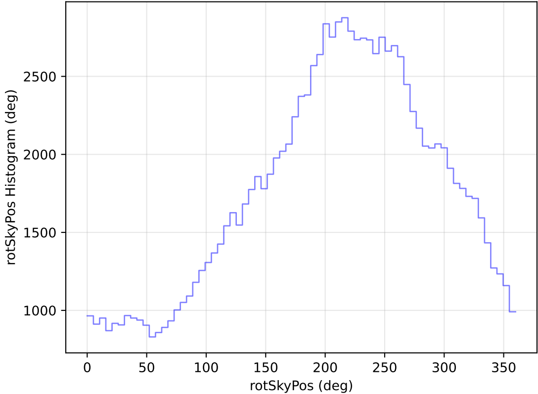
too_elab_heavy_r64_d3_ugrizy_v3.4_10yrs All sky u band: rotSkyPos Histogram
