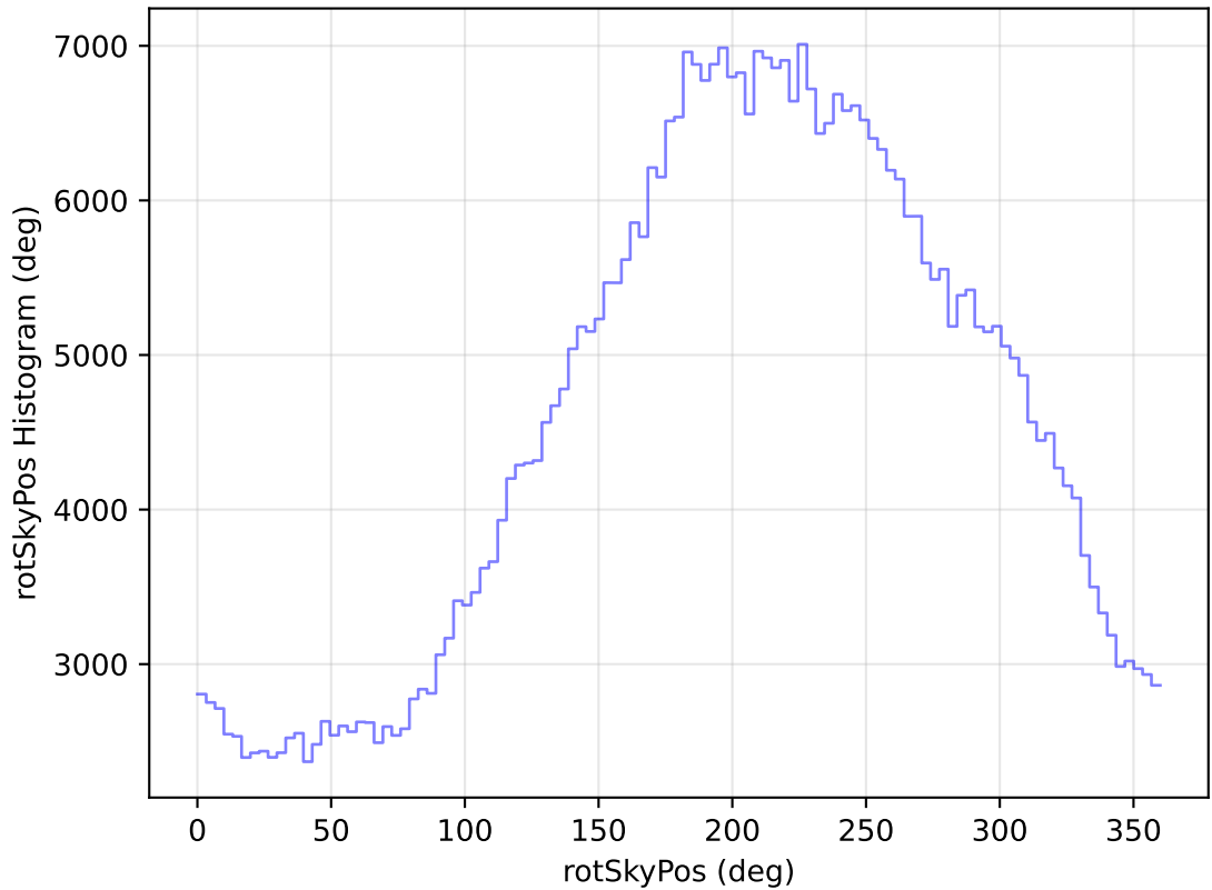
too_elab_heavy_r64_d3_ugrizy_v3.4_10yrs All sky i band: rotSkyPos Histogram
