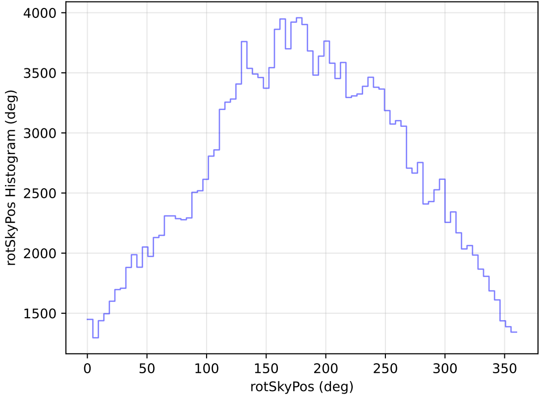
too_elab_heavy_r64_d3_ugrizy_v3.4_10yrs All sky g band: rotSkyPos Histogram
