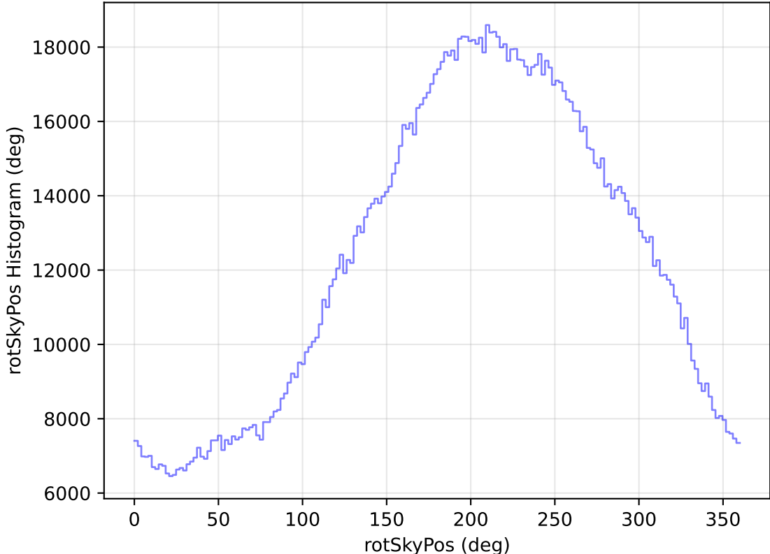
too_elab_heavy_r64_d3_ugrizy_v3.4_10yrs All sky all bands: rotSkyPos Histogram
