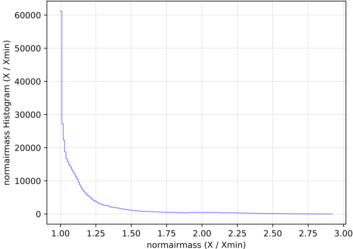
too_elab_heavy_r64_d3_ugrizy_v3.4_10yrs WFD z band: normairmass Histogram
