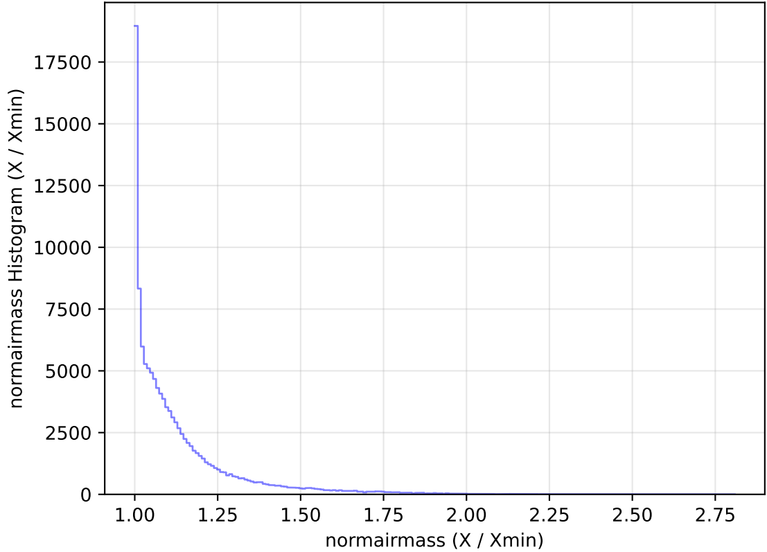
too_elab_heavy_r64_d3_ugrizy_v3.4_10yrs WFD u band: normairmass Histogram
