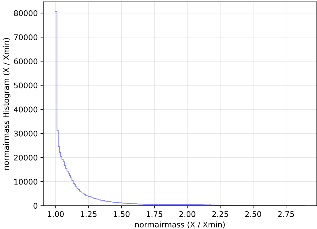
too_elab_heavy_r64_d3_ugrizy_v3.4_10yrs WFD r band: normairmass Histogram
