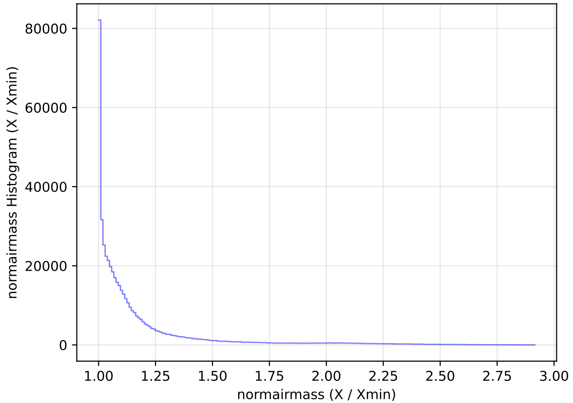
too_elab_heavy_r64_d3_ugrizy_v3.4_10yrs WFD i band: normairmass Histogram
