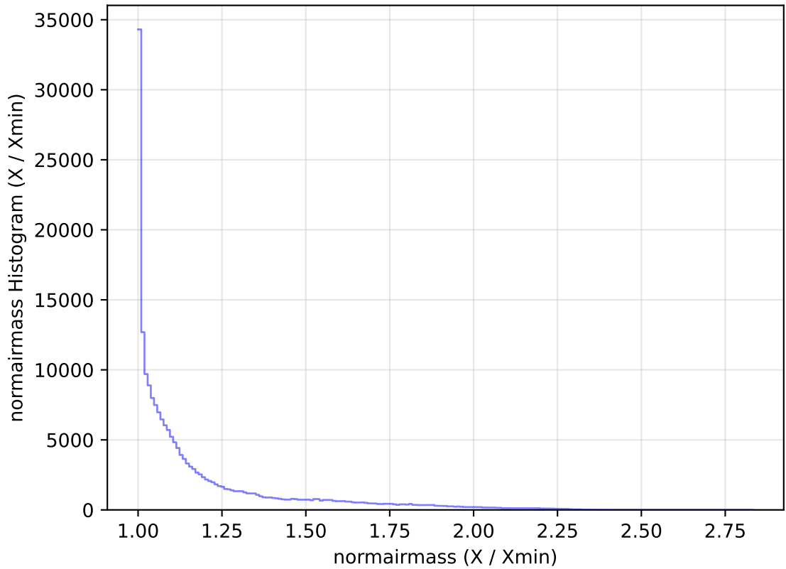
too_elab_heavy_r64_d3_ugrizy_v3.4_10yrs WFD g band: normairmass Histogram
