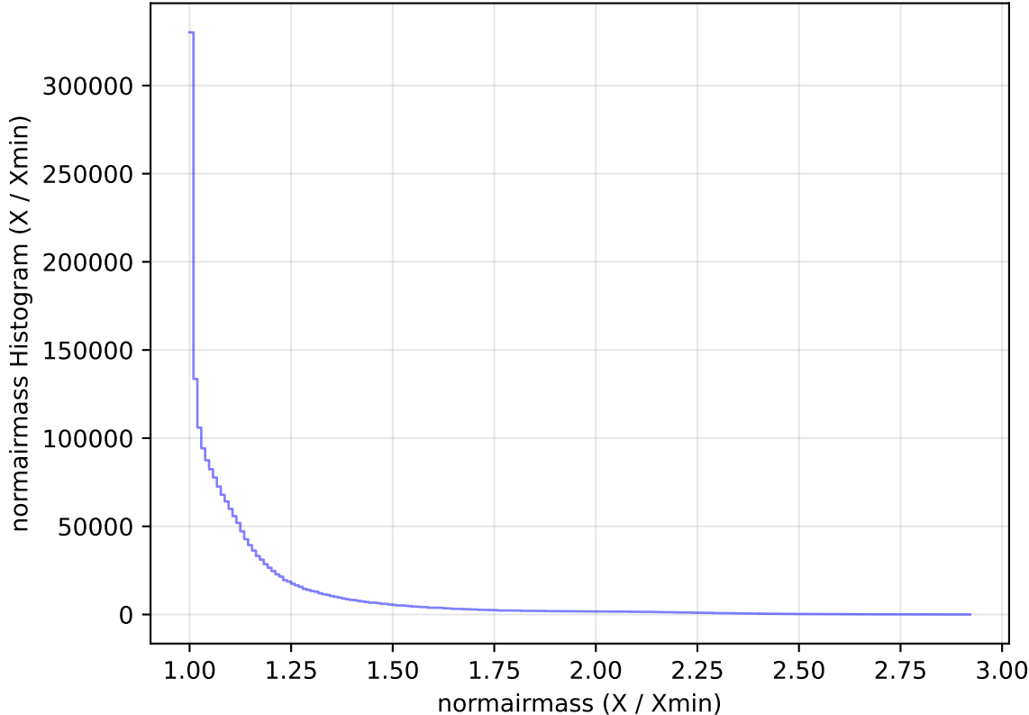
too_elab_heavy_r64_d3_ugrizy_v3.4_10yrs WFD all bands: normairmass Histogram
