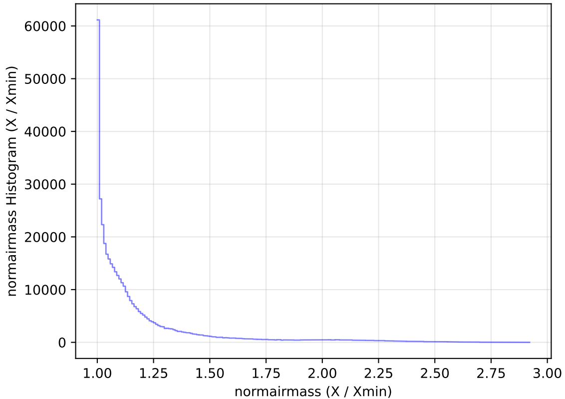
too_elab_heavy_r64_d3_ugrizy_v3.4_10yrs All sky z band: normairmass Histogram
