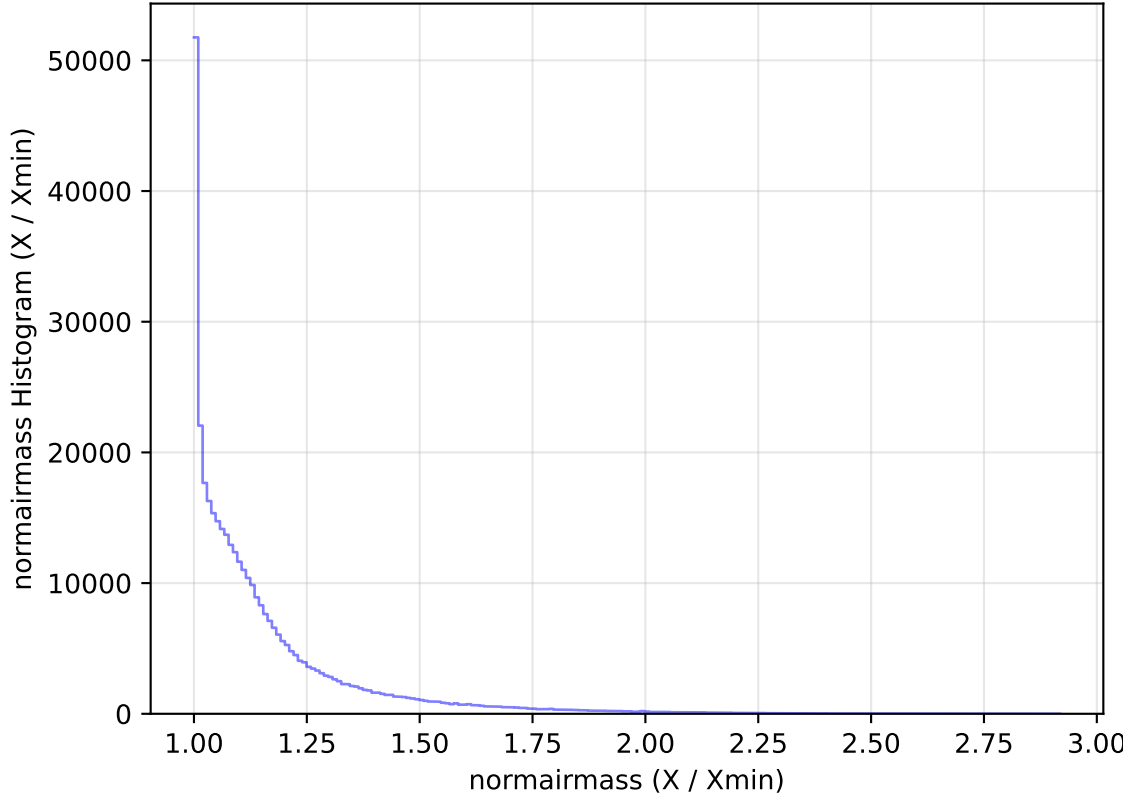
too_elab_heavy_r64_d3_ugrizy_v3.4_10yrs All sky y band: normairmass Histogram
