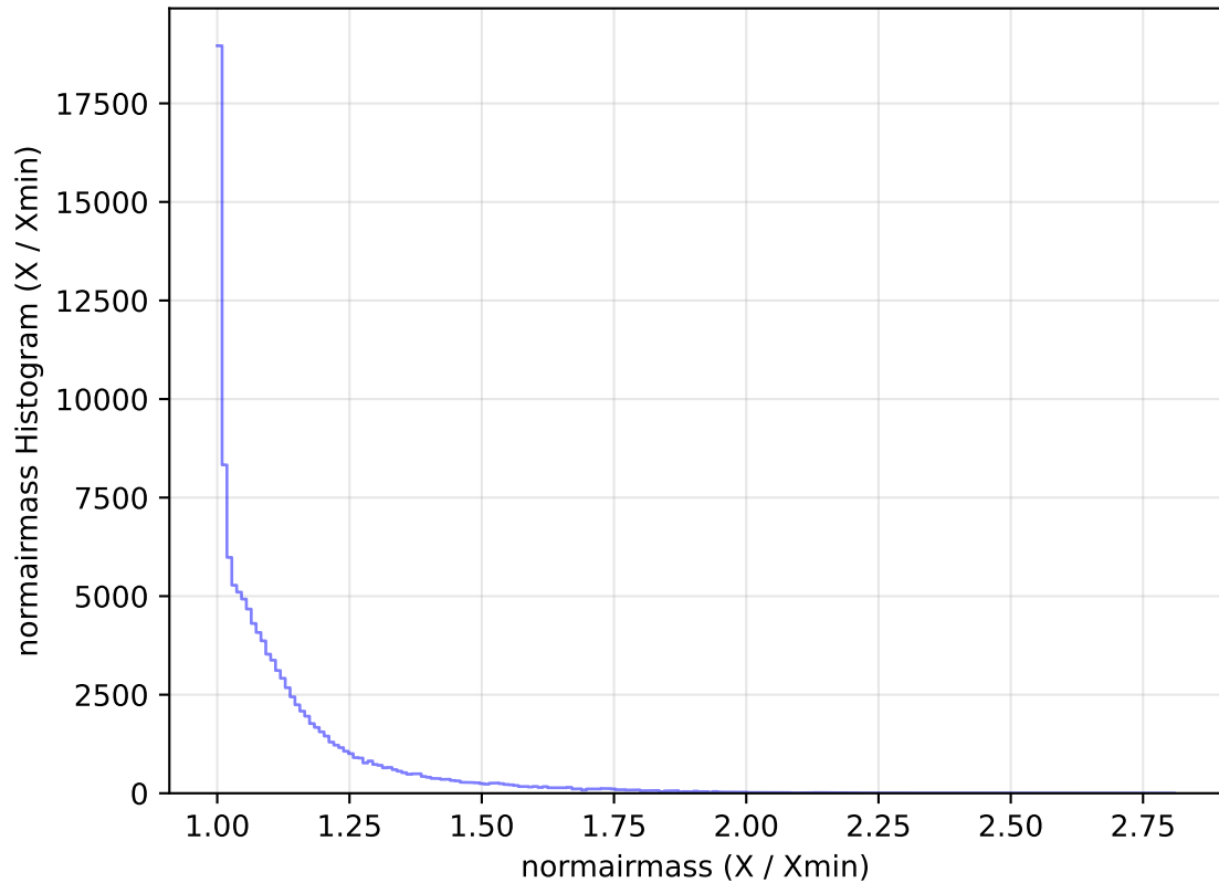
too_elab_heavy_r64_d3_ugrizy_v3.4_10yrs All sky u band: normairmass Histogram
