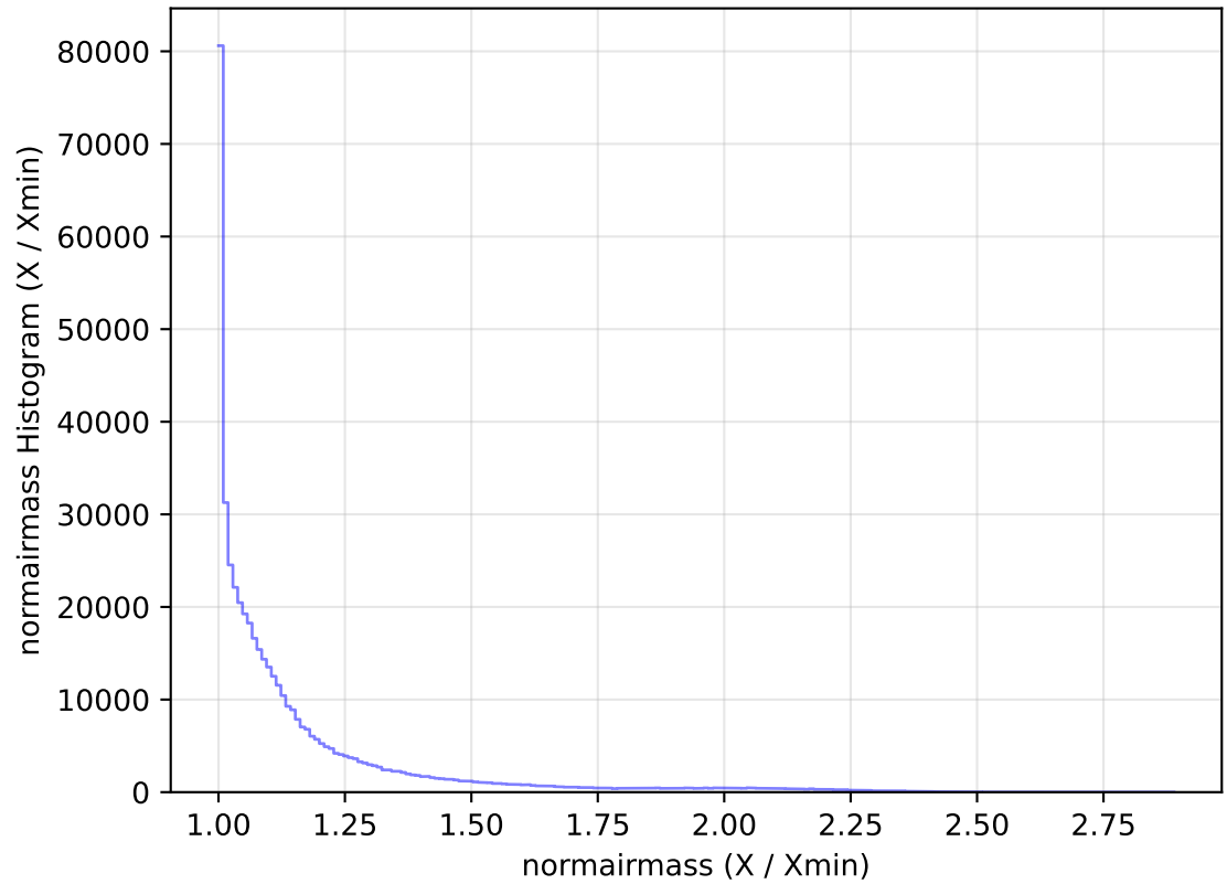
too_elab_heavy_r64_d3_ugrizy_v3.4_10yrs All sky r band: normairmass Histogram
