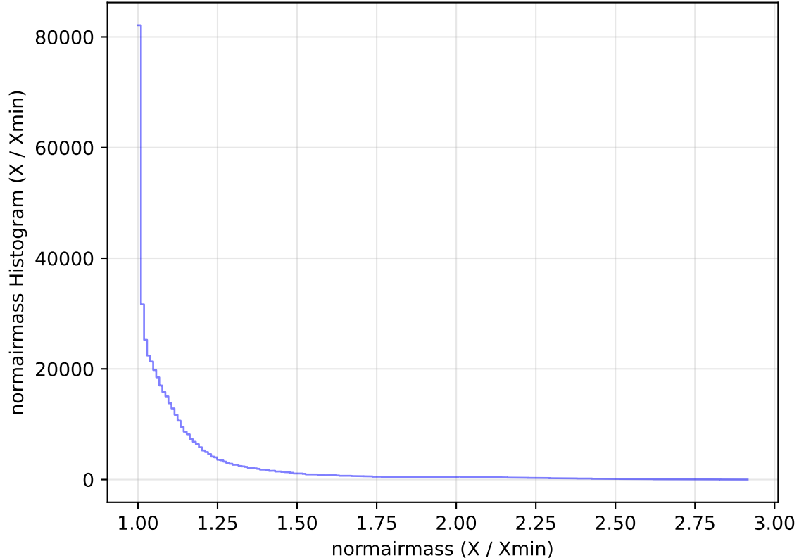
too_elab_heavy_r64_d3_ugrizy_v3.4_10yrs All sky i band: normairmass Histogram
