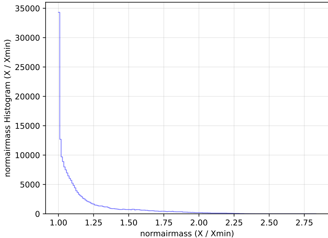
too_elab_heavy_r64_d3_ugrizy_v3.4_10yrs All sky g band: normairmass Histogram
