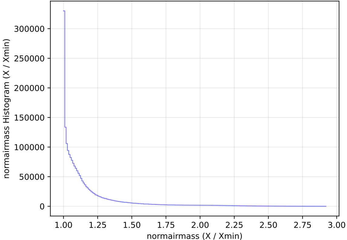
too_elab_heavy_r64_d3_ugrizy_v3.4_10yrs All sky all bands: normairmass Histogram
