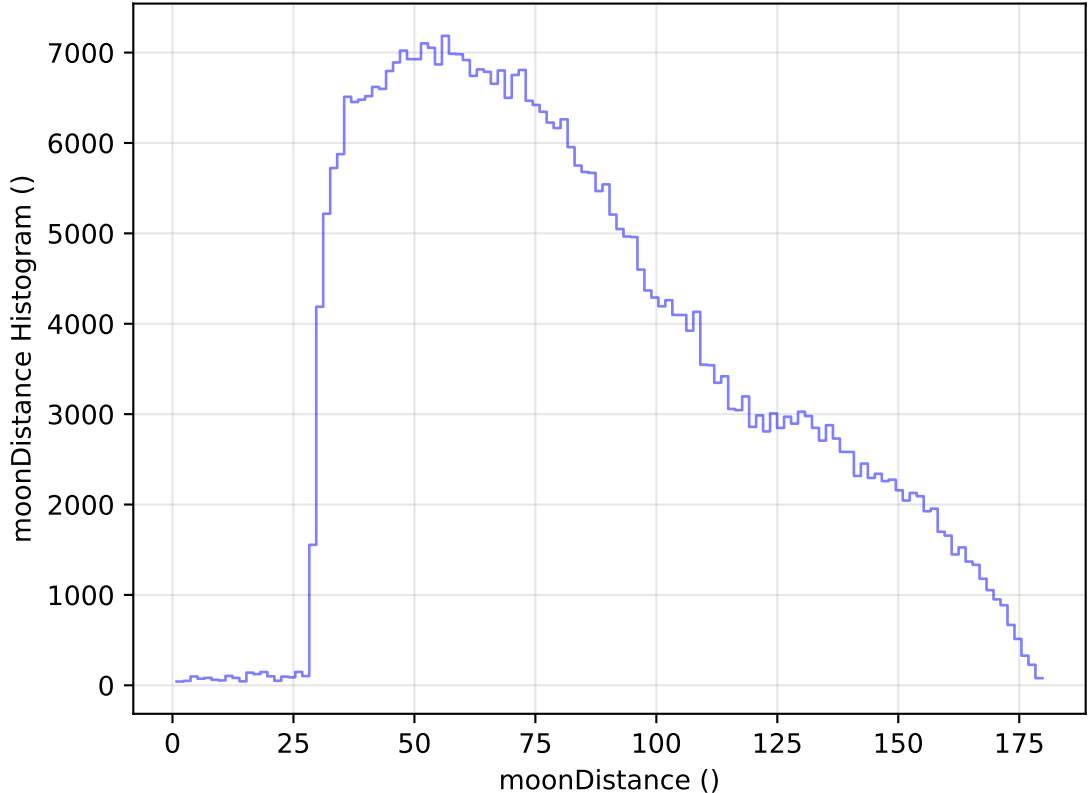
too_elab_heavy_r64_d3_ugrizy_v3.4_10yrs WFD z band: moonDistance Histogram
