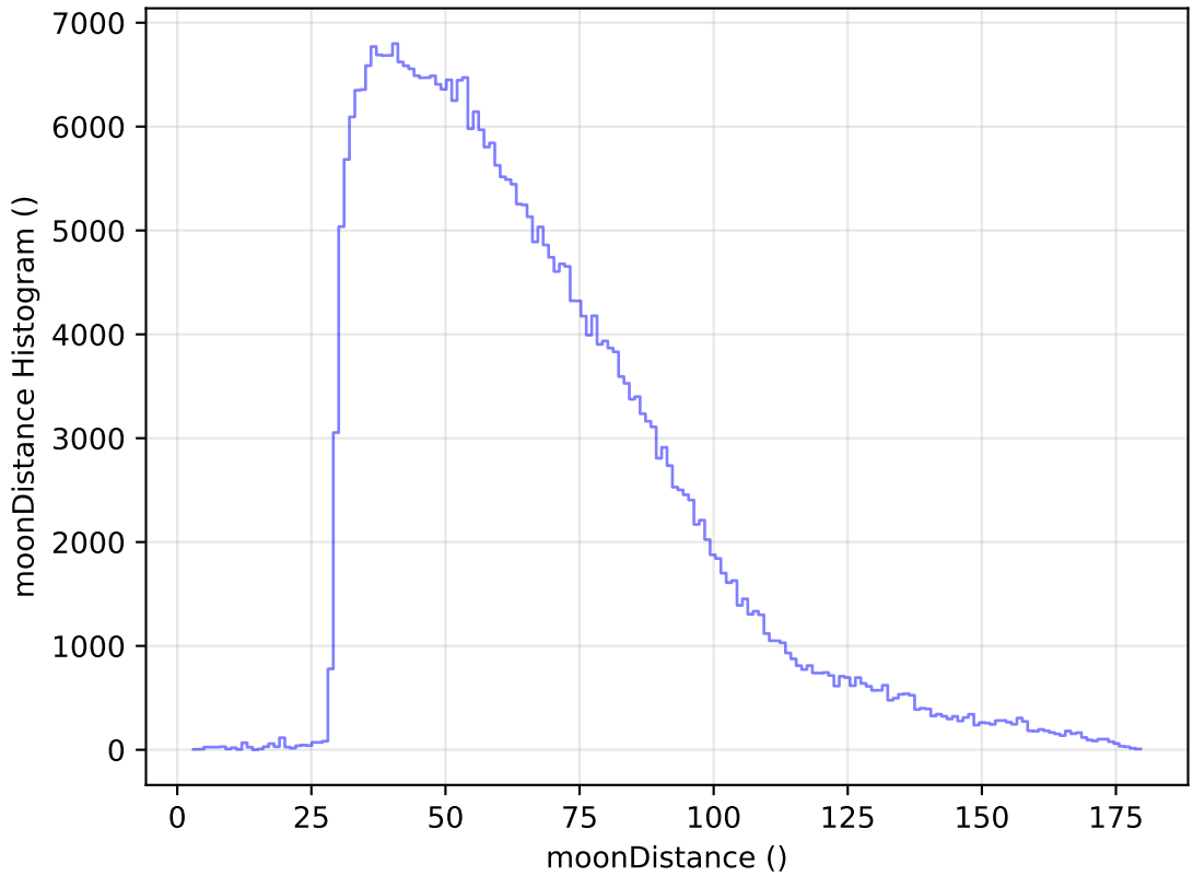
too_elab_heavy_r64_d3_ugrizy_v3.4_10yrs WFD y band: moonDistance Histogram
