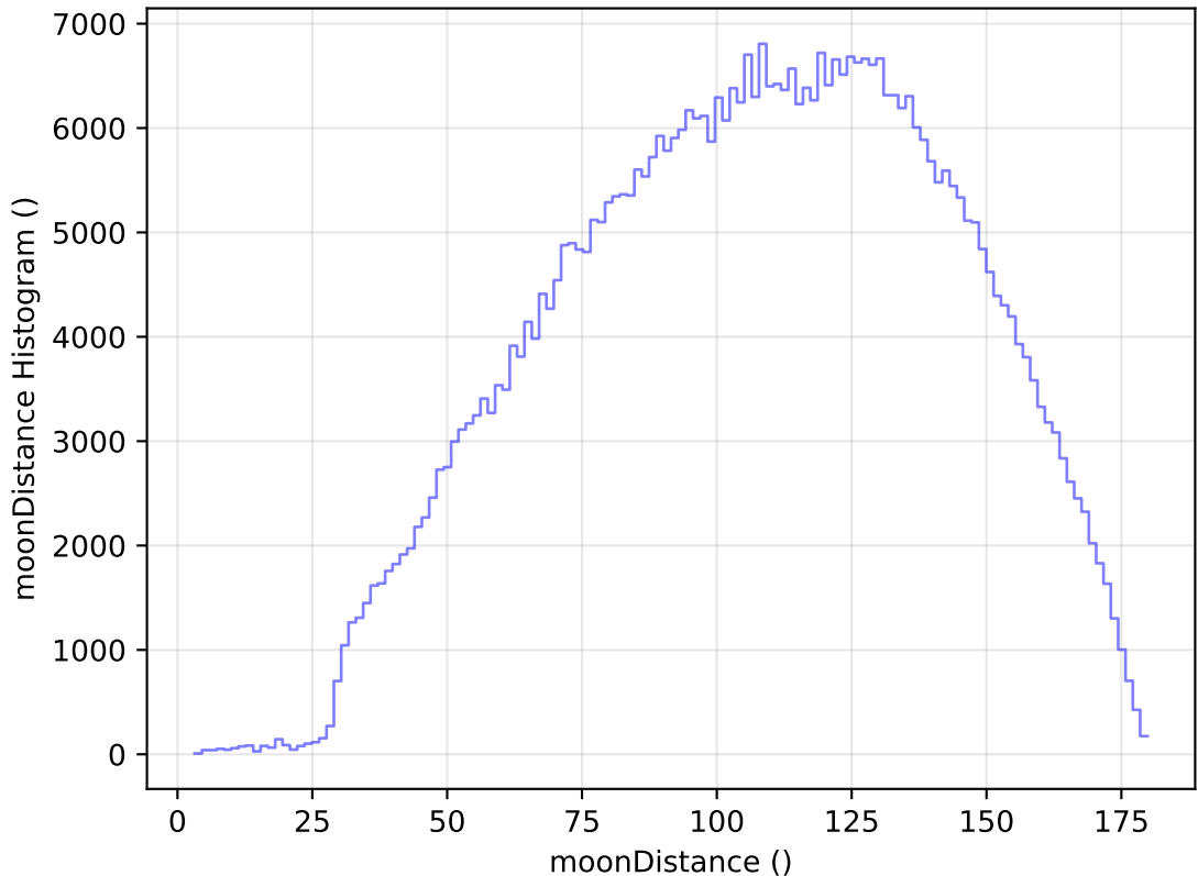
too_elab_heavy_r64_d3_ugrizy_v3.4_10yrs WFD r band: moonDistance Histogram
