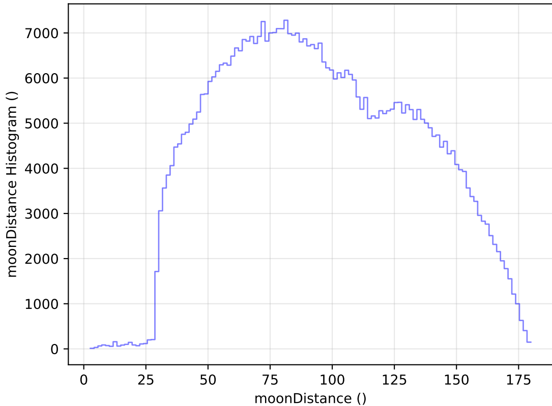
too_elab_heavy_r64_d3_ugrizy_v3.4_10yrs WFD i band: moonDistance Histogram
