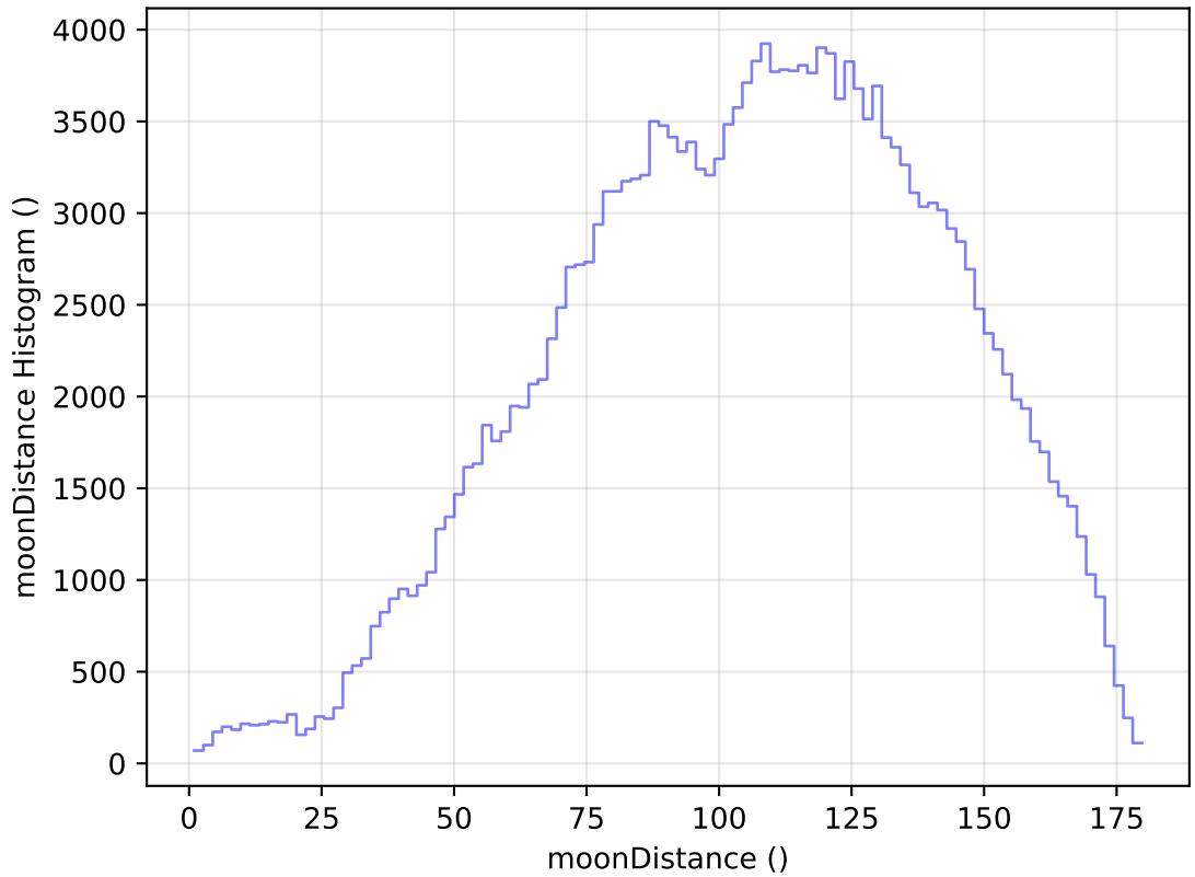
too_elab_heavy_r64_d3_ugrizy_v3.4_10yrs WFD g band: moonDistance Histogram
