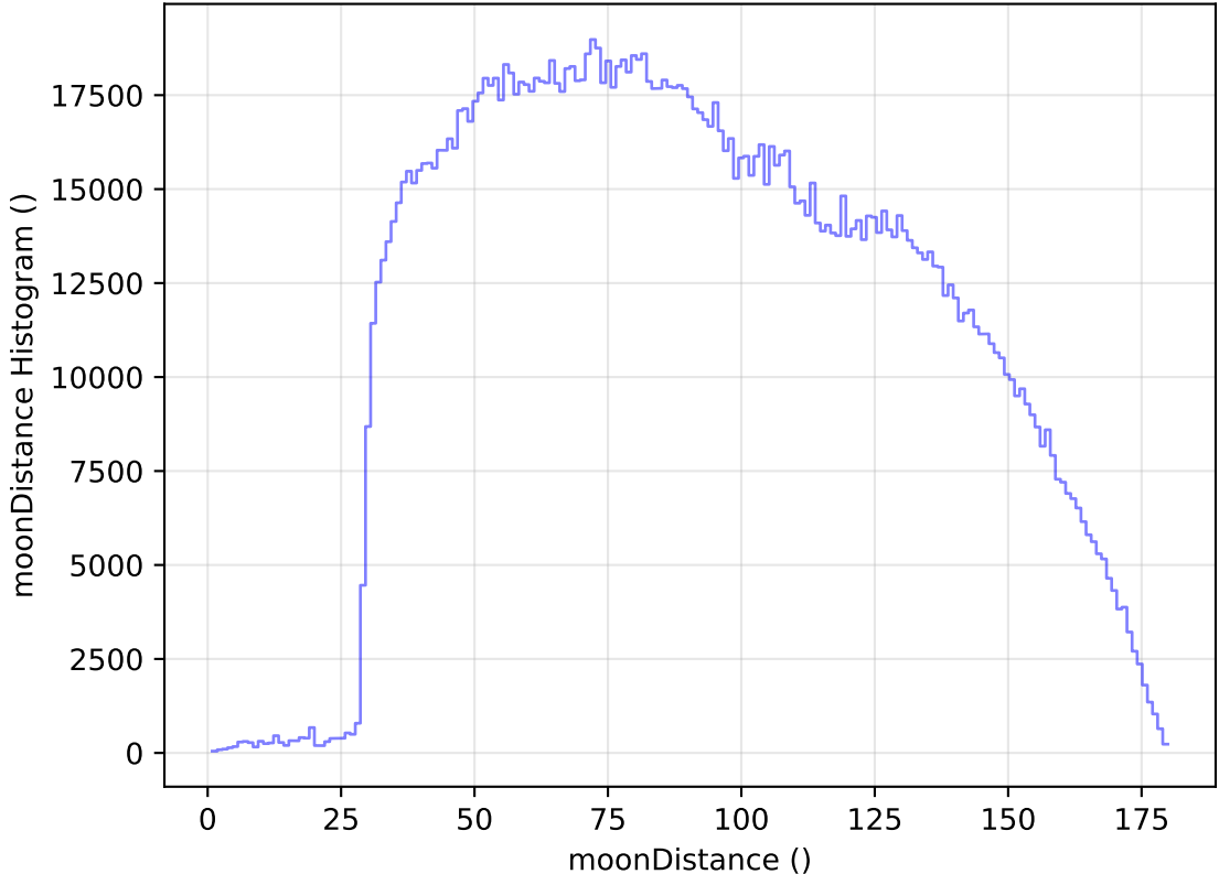
too_elab_heavy_r64_d3_ugrizy_v3.4_10yrs WFD all bands: moonDistance Histogram
