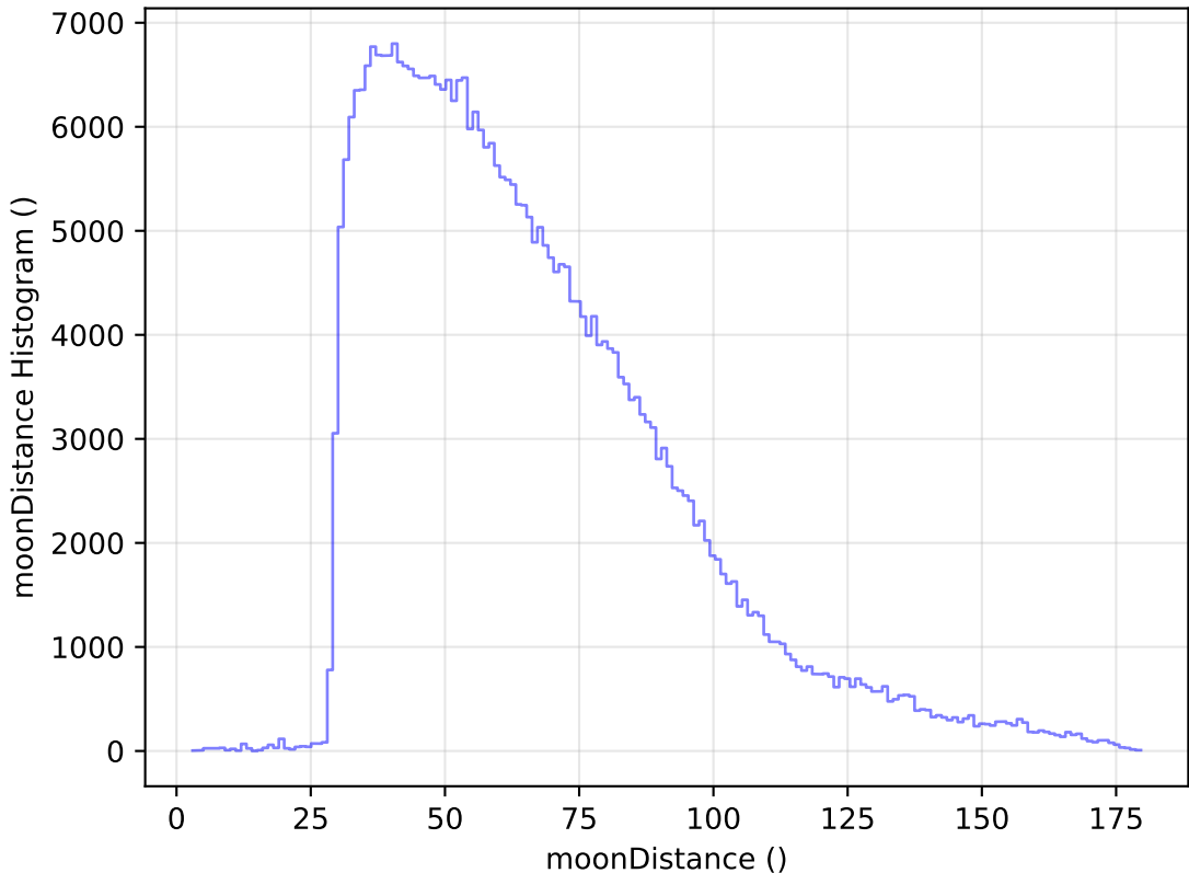
too_elab_heavy_r64_d3_ugrizy_v3.4_10yrs All sky y band: moonDistance Histogram
