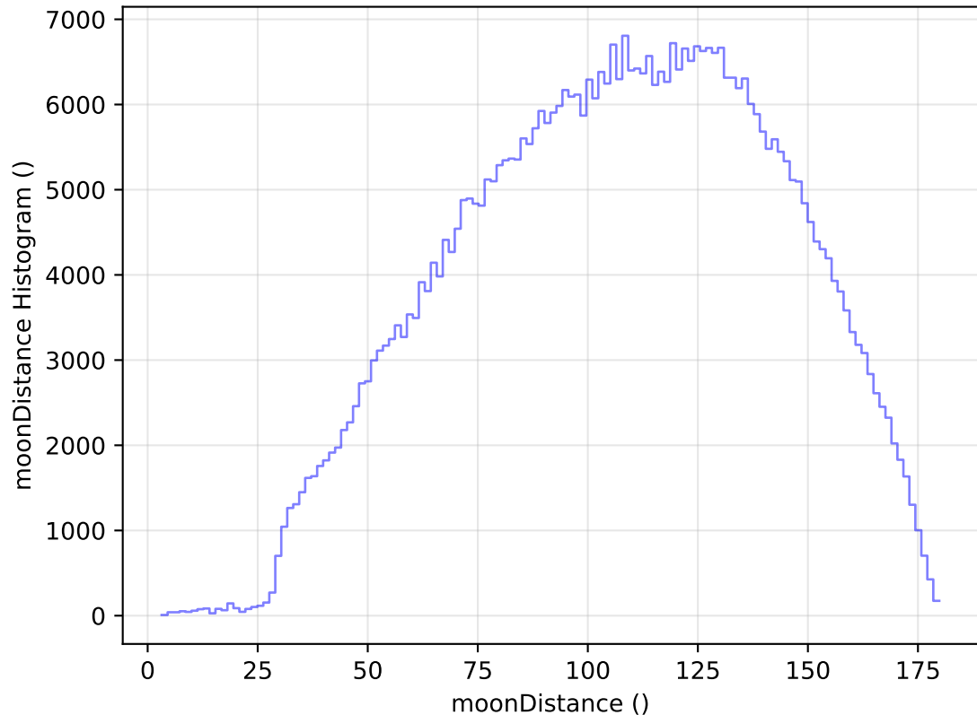
too_elab_heavy_r64_d3_ugrizy_v3.4_10yrs All sky r band: moonDistance Histogram
