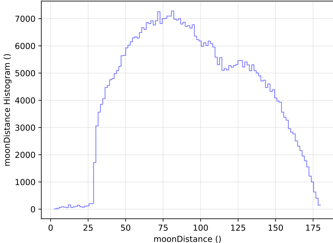
too_elab_heavy_r64_d3_ugrizy_v3.4_10yrs All sky i band: moonDistance Histogram
