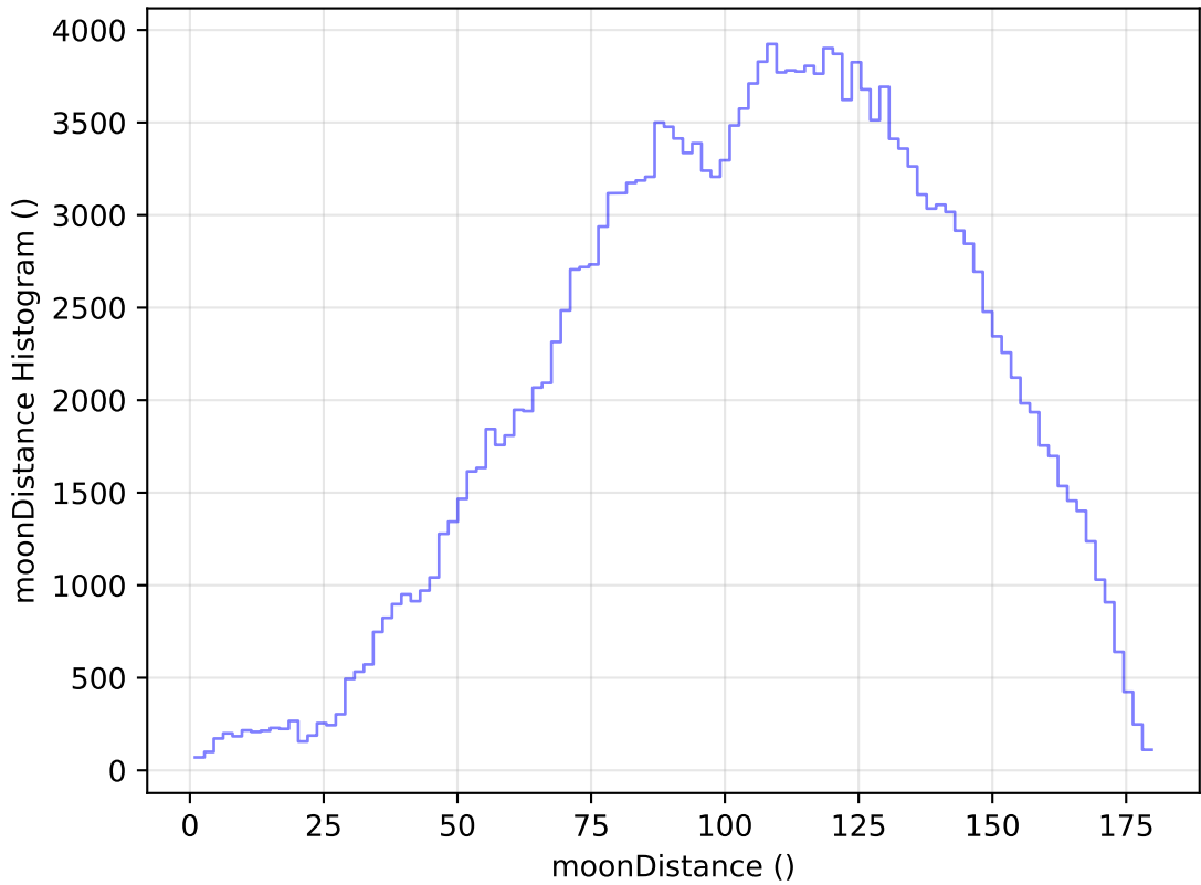
too_elab_heavy_r64_d3_ugrizy_v3.4_10yrs All sky g band: moonDistance Histogram
