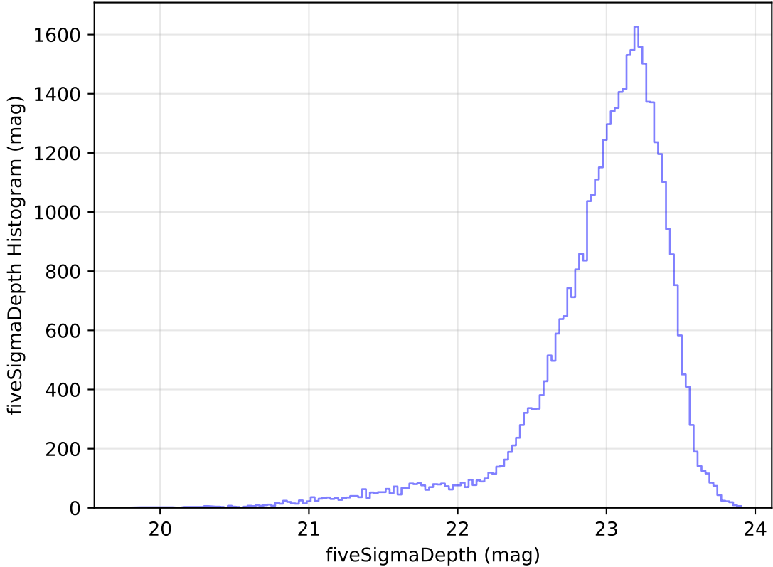
too_elab_heavy_r64_d3_ugrizy_v3.4_10yrs Yr 1 z band: fiveSigmaDepth Histogram
