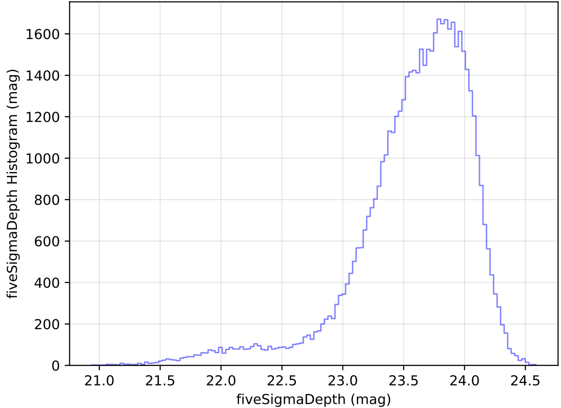
too_elab_heavy_r64_d3_ugrizy_v3.4_10yrs Yr 1 i band: fiveSigmaDepth Histogram
