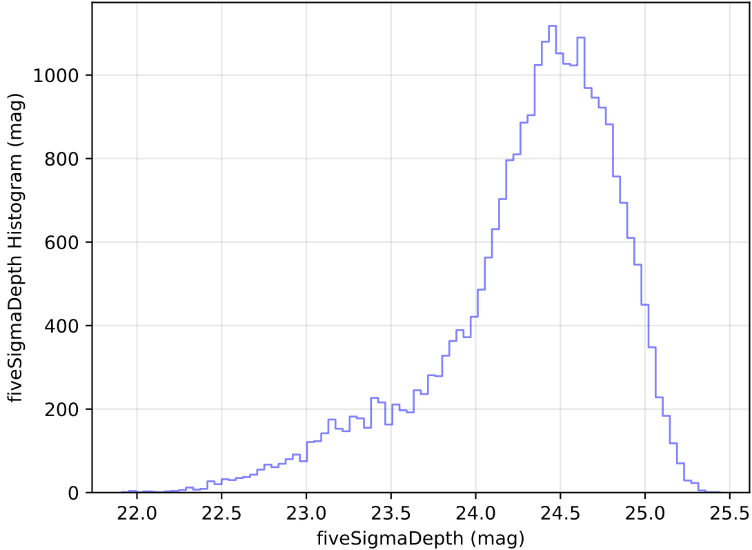
too_elab_heavy_r64_d3_ugrizy_v3.4_10yrs Yr 1 g band: fiveSigmaDepth Histogram
