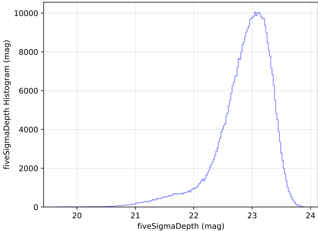
too_elab_heavy_r64_d3_ugrizy_v3.4_10yrs WFD z band: fiveSigmaDepth Histogram
